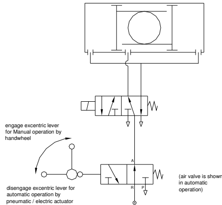
fig 2.1 double acting
