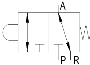
Figure 5: port designation
