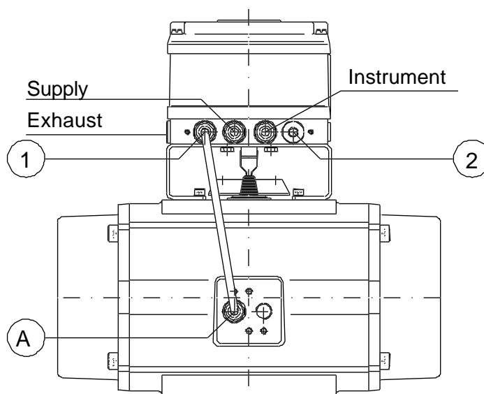
Pneumatic Connections Single acting
