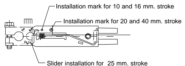
b) Lever for 10 to 40 mm. Stroke
