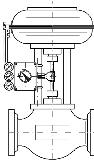
Double acting
